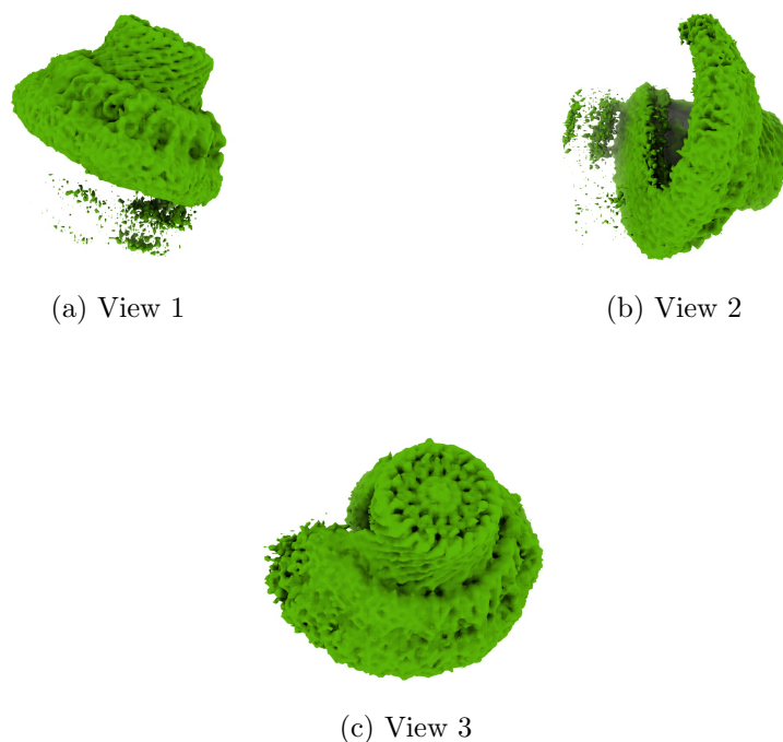
Figure 4: Isosurface at threshold=0.053600. Views generated by ChimeraX at a the following X, Y, Z angles: View 1 (0, -90, -90), View 2 (-90, 0, -90), View 3 (0, 0, 0).
