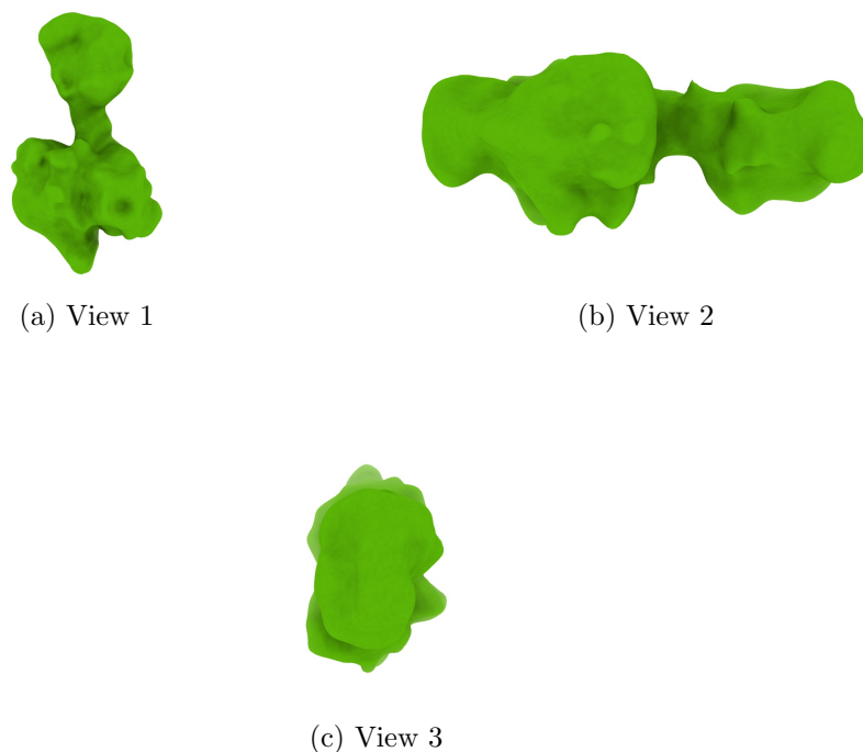
Figure 4: Isosurface at threshold=0.007300. Views generated by ChimeraX at a the following X, Y, Z angles: View 1 (0, -90, -90), View 2 (-90, 0, -90), View 3 (0, 0, 0).
