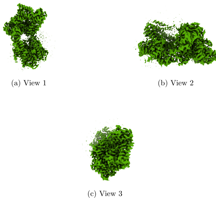
Figure 4: Isosurface at threshold=1.460000. Views generated by ChimeraX at a the following X, Y, Z angles: View 1 (0, -90, -90), View 2 (-90, 0, -90), View 3 (0, 0, 0).
