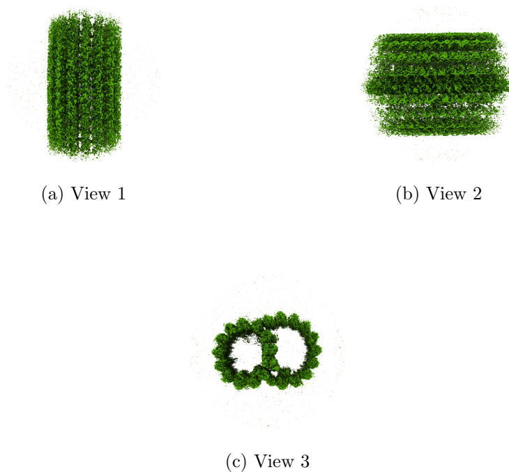
Figure 4: Isosurface at threshold=0.083600. Views generated by ChimeraX at a the following X, Y, Z angles: View 1 (0, -90, -90), View 2 (-90, 0, -90), View 3 (0, 0, 0).
