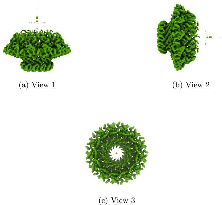
Figure 4: Isosurface at threshold=0.093400. Views generated by ChimeraX at a the following X, Y, Z angles: View 1 (0, -90, -90), View 2 (-90, 0, -90), View 3 (0, 0, 0).
