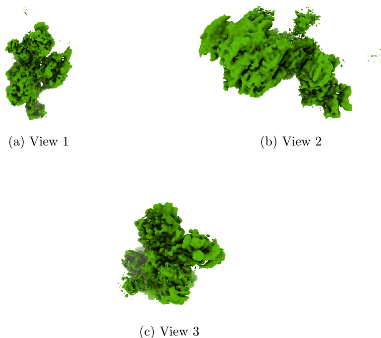
Figure 4: Isosurface at threshold=0.005200. Views generated by ChimeraX at a the following X, Y, Z angles: View 1 (0, -90, -90), View 2 (-90, 0, -90), View 3 (0, 0, 0).
