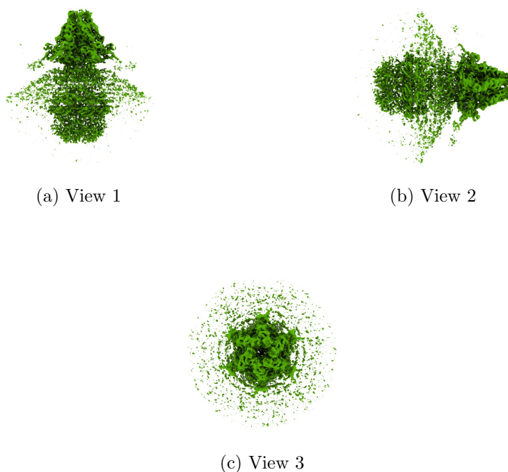
Figure 4: Isosurface at threshold=0.191000. Views generated by ChimeraX at a the following X, Y, Z angles: View 1 (0, -90, -90), View 2 (-90, 0, -90), View 3 (0, 0, 0).
