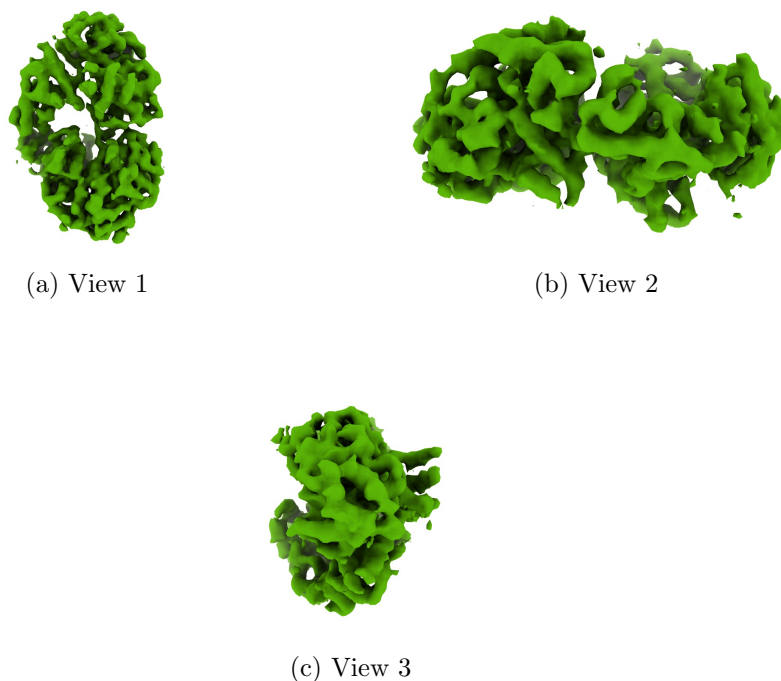
Figure 4: Isosurface at threshold=0.876000. Views generated by ChimeraX at a the following X, Y, Z angles: View 1 (0, -90, -90), View 2 (-90, 0, -90), View 3 (0, 0, 0).
