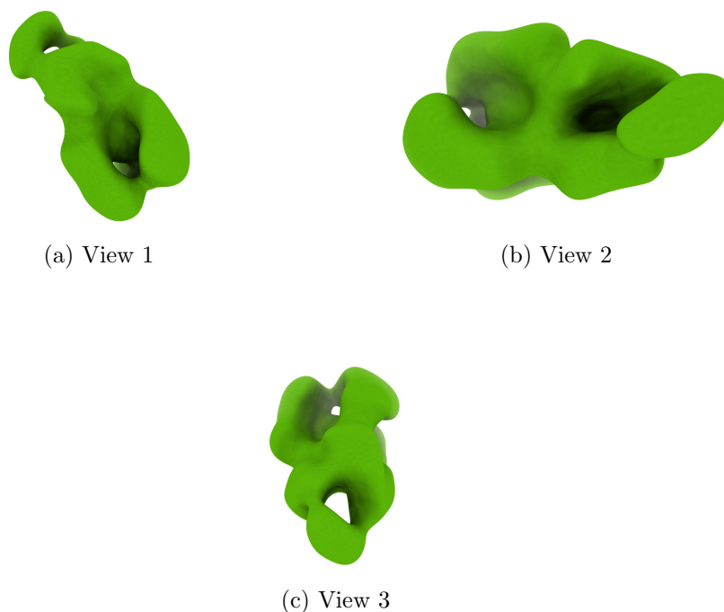
Figure 4: Isosurface at threshold=0.009170. Views generated by ChimeraX at a the following X, Y, Z angles: View 1 (0, -90, -90), View 2 (-90, 0, -90), View 3 (0, 0, 0).
