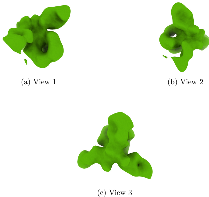
Figure 4: Isosurface at threshold=0.006630. Views generated by ChimeraX at a the following X, Y, Z angles: View 1 (0, -90, -90), View 2 (-90, 0, -90), View 3 (0, 0, 0).
