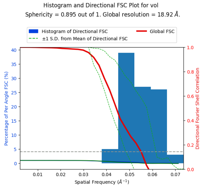
Figure 27: Global FSC and histogram of the directional FSC.
