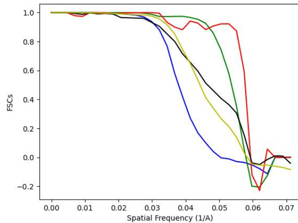
Figure 26: FSC in X, Y, Z, the global FSC, and the Average Cosine Phase.
