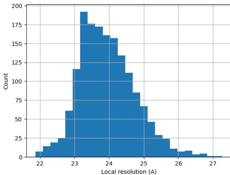
Figure 20: Histogram of the local resolution according to blocres.
