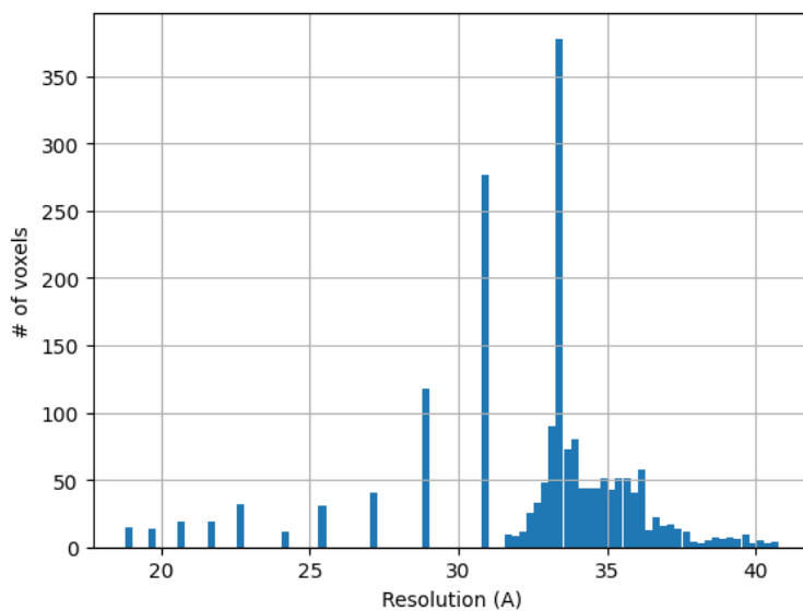
Figure 22: Histogram of the local resolution according to MonoRes.
