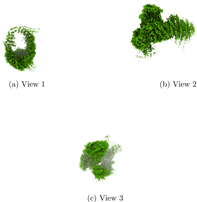
Figure 4: Isosurface at threshold=0.055000. Views generated by ChimeraX at a the following X, Y, Z angles: View 1 (0, -90, -90), View 2 (-90, 0, -90), View 3 (0, 0, 0).
