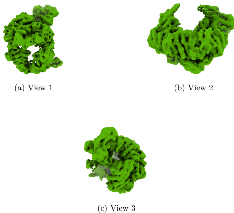
Figure 4: Isosurface at threshold=0.116000. Views generated by ChimeraX at a the following X, Y, Z angles: View 1 (0, -90, -90), View 2 (-90, 0, -90), View 3 (0, 0, 0).
