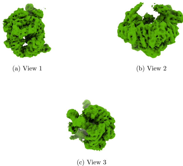
Figure 4: Isosurface at threshold=0.088200. Views generated by ChimeraX at a the following X, Y, Z angles: View 1 (0, -90, -90), View 2 (-90, 0, -90), View 3 (0, 0, 0).
