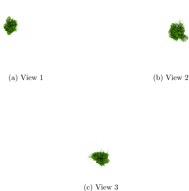
Figure 4: Isosurface at threshold=1.200000. Views generated by ChimeraX at a the following X, Y, Z angles: View 1 (0, -90, -90), View 2 (-90, 0, -90), View 3 (0, 0, 0).
