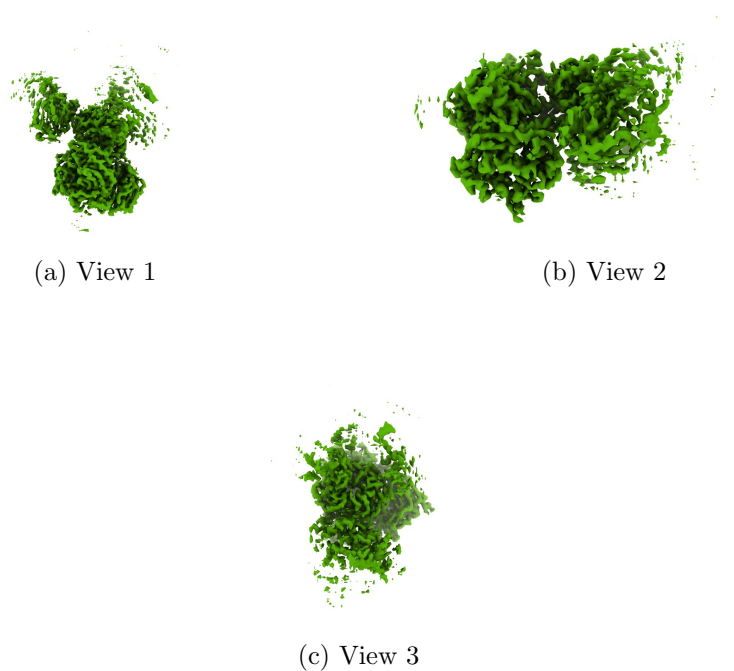
Figure 4: Isosurface at threshold=0.055400. Views generated by ChimeraX at a the following X, Y, Z angles: View 1 (0, -90, -90), View 2 (-90, 0, -90), View 3 (0, 0, 0).
