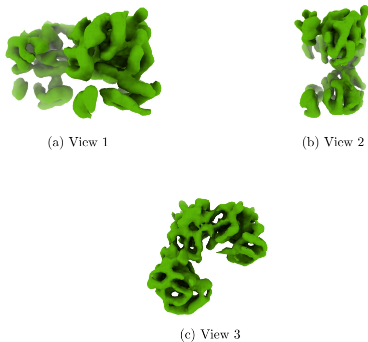
Figure 4: Isosurface at threshold=0.215000. Views generated by ChimeraX at a the following X, Y, Z angles: View 1 (0, -90, -90), View 2 (-90, 0, -90), View 3 (0, 0, 0).
