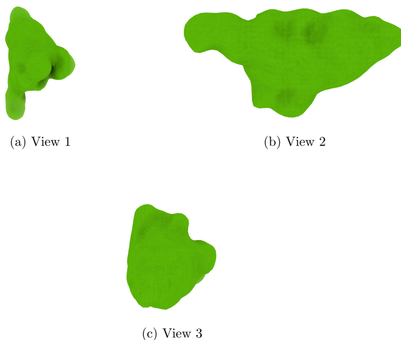
Figure 4: Isosurface at threshold=2.930000. Views generated by ChimeraX at a the following X, Y, Z angles: View 1 (0, -90, -90), View 2 (-90, 0, -90), View 3 (0, 0, 0).
