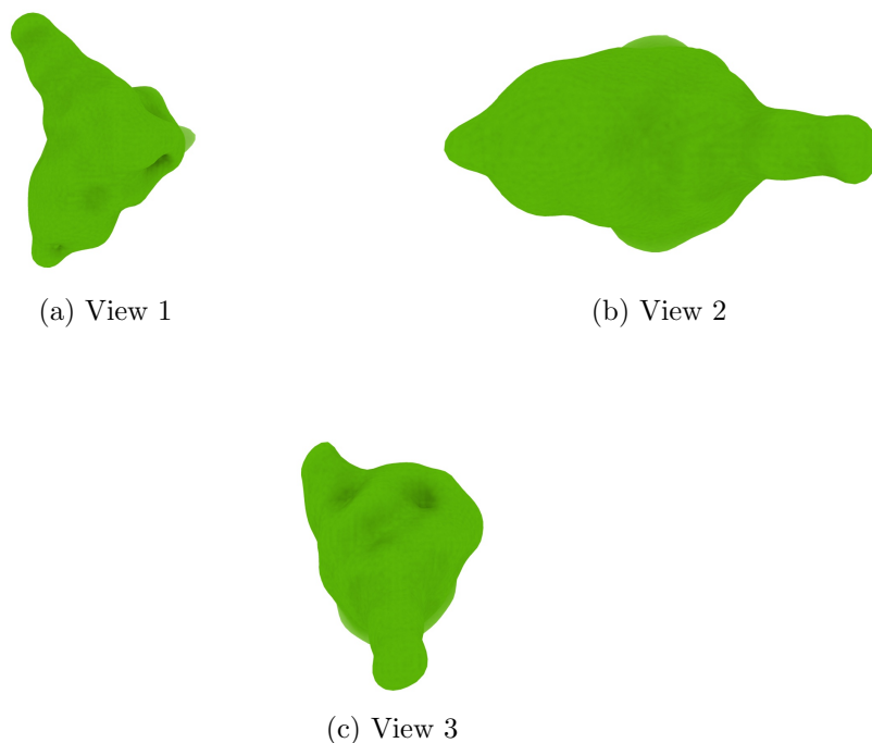
Figure 4: Isosurface at threshold=1.510000. Views generated by ChimeraX at a the following X, Y, Z angles: View 1 (0, -90, -90), View 2 (-90, 0, -90), View 3 (0, 0, 0).
