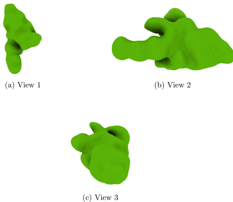
Figure 4: Isosurface at threshold=1.130000. Views generated by ChimeraX at a the following X, Y, Z angles: View 1 (0, -90, -90), View 2 (-90, 0, -90), View 3 (0, 0, 0).
