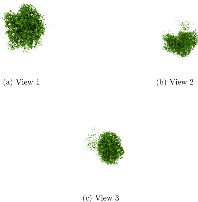
Figure 4: Isosurface at threshold=0.127000. Views generated by ChimeraX at a the following X, Y, Z angles: View 1 (0, -90, -90), View 2 (-90, 0, -90), View 3 (0, 0, 0).
