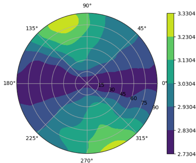
Figure 27: Directional resolution in the projection sphere.
