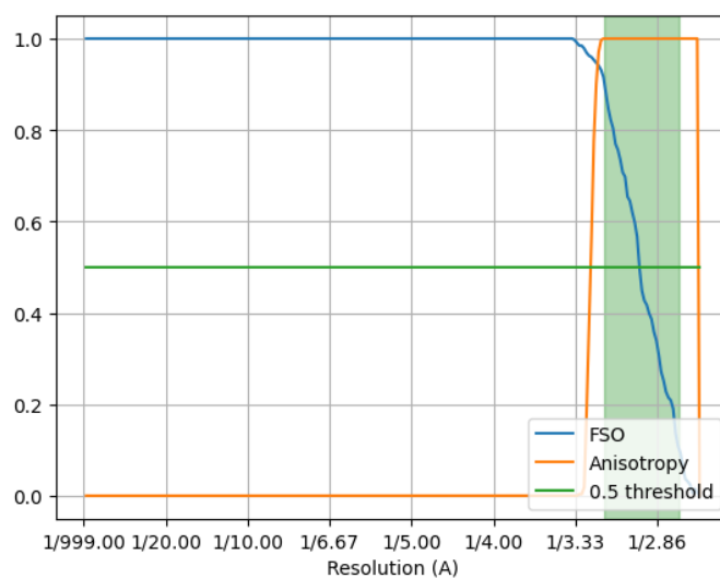
Figure 26: FSO and anisotropy.
