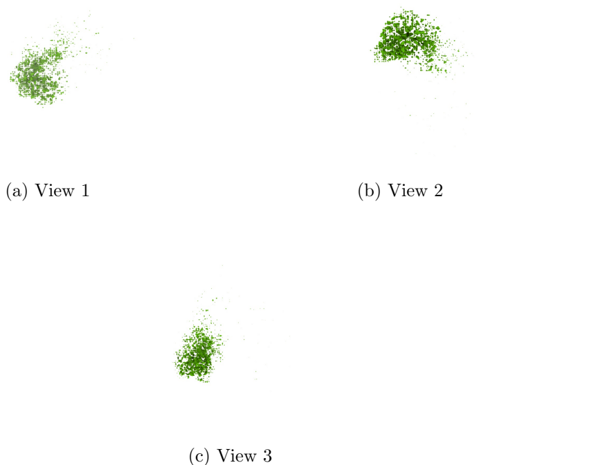
Figure 4: Isosurface at threshold=0.130000. Views generated by ChimeraX at a the following X, Y, Z angles: View 1 (0, -90, -90), View 2 (-90, 0, -90), View 3 (0, 0, 0).
