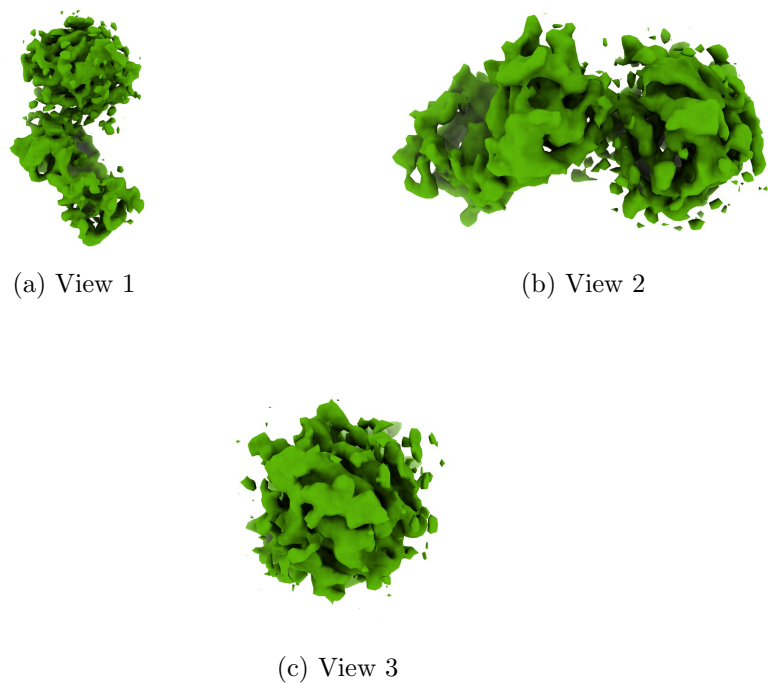
Figure 4: Isosurface at threshold=1.430000. Views generated by ChimeraX at a the following X, Y, Z angles: View 1 (0, -90, -90), View 2 (-90, 0, -90), View 3 (0, 0, 0).
