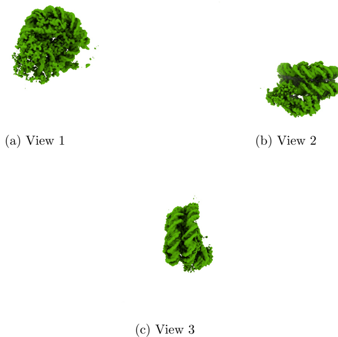
Figure 4: Isosurface at threshold=0.017600. Views generated by ChimeraX at a the following X, Y, Z angles: View 1 (0, -90, -90), View 2 (-90, 0, -90), View 3 (0, 0, 0).
