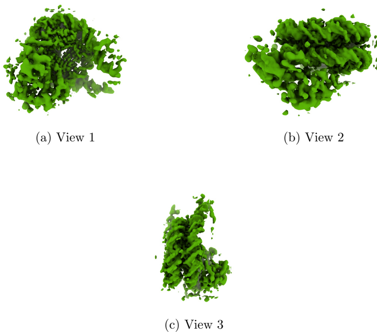
Figure 4: Isosurface at threshold=0.075400. Views generated by ChimeraX at a the following X, Y, Z angles: View 1 (0, -90, -90), View 2 (-90, 0, -90), View 3 (0, 0, 0).
