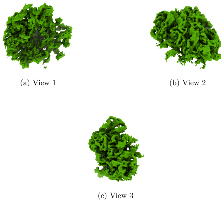
Figure 4: Isosurface at threshold=0.304000. Views generated by ChimeraX at a the following X, Y, Z angles: View 1 (0, -90, -90), View 2 (-90, 0, -90), View 3 (0, 0, 0).
