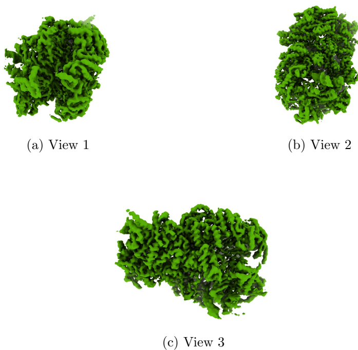
Figure 4: Isosurface at threshold=0.237000. Views generated by ChimeraX at a the following X, Y, Z angles: View 1 (0, -90, -90), View 2 (-90, 0, -90), View 3 (0, 0, 0).
