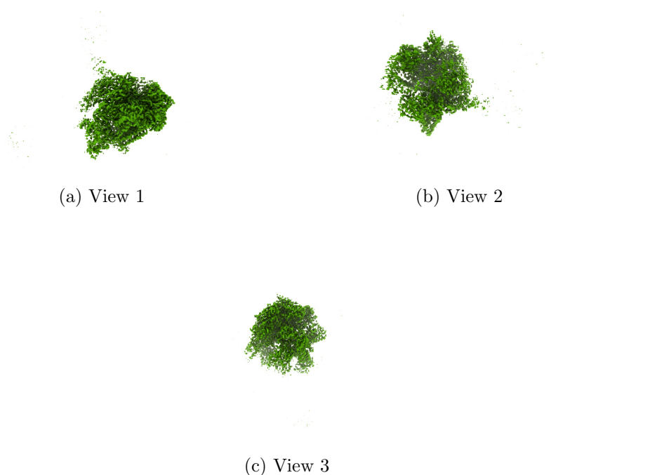
Figure 4: Isosurface at threshold=0.343000. Views generated by ChimeraX at a the following X, Y, Z angles: View 1 (0, -90, -90), View 2 (-90, 0, -90), View 3 (0, 0, 0).
