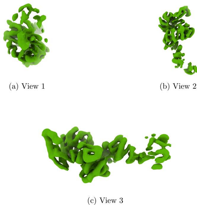
Figure 4: Isosurface at threshold=0.150000. Views generated by ChimeraX at a the following X, Y, Z angles: View 1 (0, -90, -90), View 2 (-90, 0, -90), View 3 (0, 0, 0).
