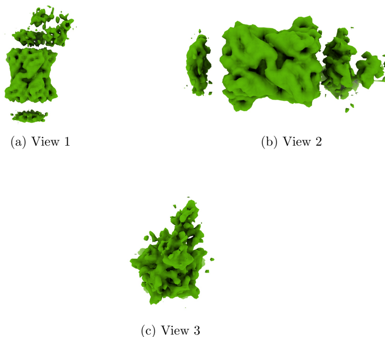
Figure 4: Isosurface at threshold=0.042400. Views generated by ChimeraX at a the following X, Y, Z angles: View 1 (0, -90, -90), View 2 (-90, 0, -90), View 3 (0, 0, 0).
