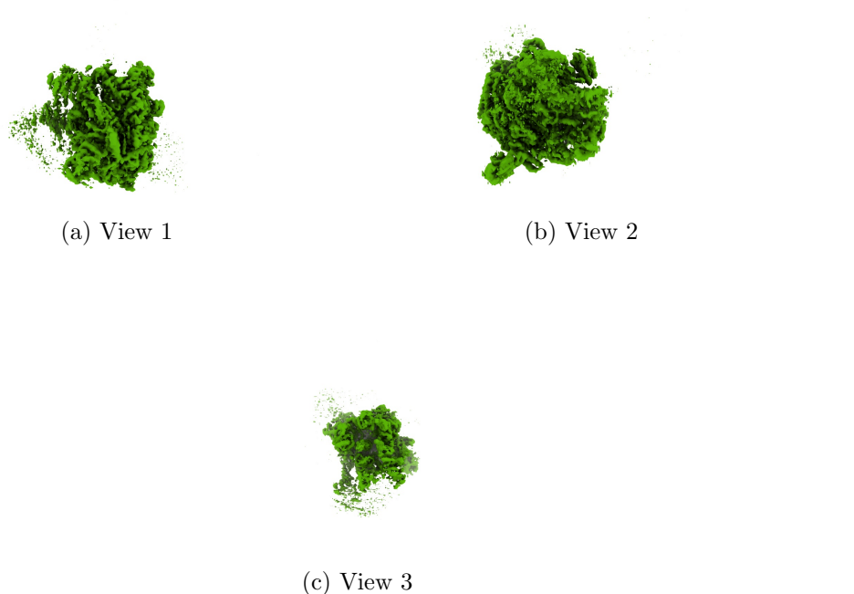
Figure 4: Isosurface at threshold=0.050000. Views generated by ChimeraX at a the following X, Y, Z angles: View 1 (0, -90, -90), View 2 (-90, 0, -90), View 3 (0, 0, 0).
