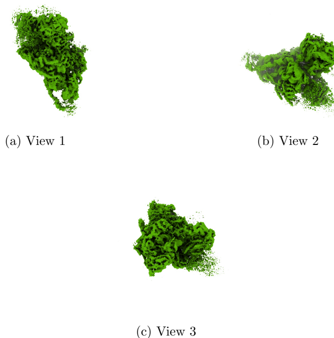
Figure 4: Isosurface at threshold=0.403000. Views generated by ChimeraX at a the following X, Y, Z angles: View 1 (0, -90, -90), View 2 (-90, 0, -90), View 3 (0, 0, 0).
