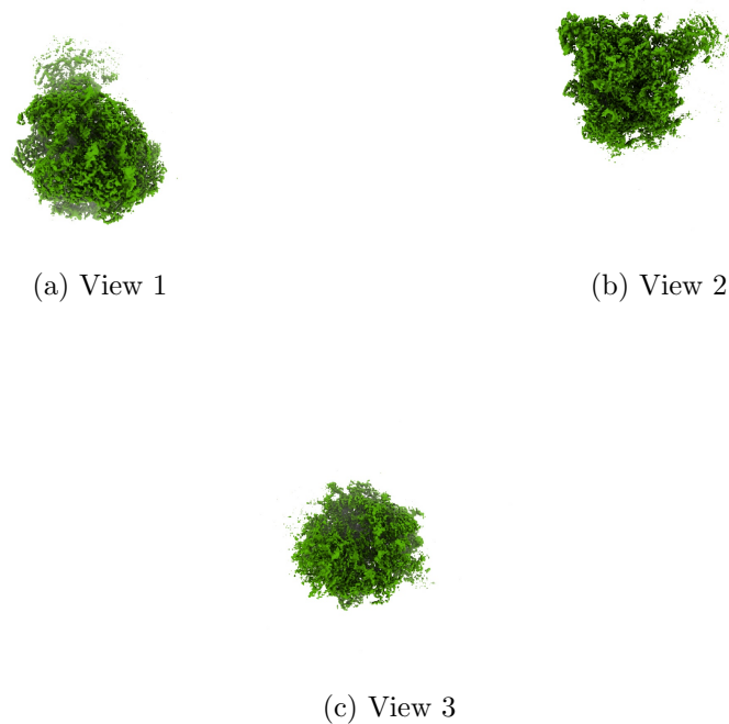
Figure 4: Isosurface at threshold=0.859000. Views generated by ChimeraX at a the following X, Y, Z angles: View 1 (0, -90, -90), View 2 (-90, 0, -90), View 3 (0, 0, 0).
