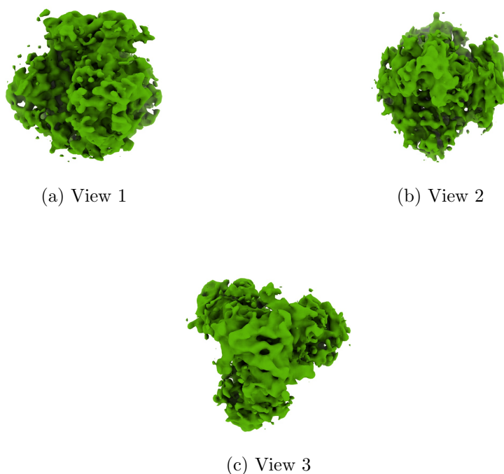
Figure 4: Isosurface at threshold=0.041700. Views generated by ChimeraX at a the following X, Y, Z angles: View 1 (0, -90, -90), View 2 (-90, 0, -90), View 3 (0, 0, 0).
