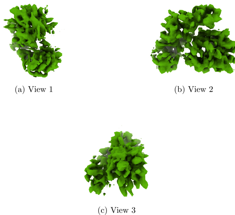
Figure 4: Isosurface at threshold=0.422000. Views generated by ChimeraX at a the following X, Y, Z angles: View 1 (0, -90, -90), View 2 (-90, 0, -90), View 3 (0, 0, 0).
