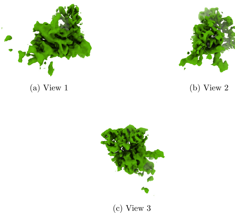
Figure 4: Isosurface at threshold=0.241000. Views generated by ChimeraX at a the following X, Y, Z angles: View 1 (0, -90, -90), View 2 (-90, 0, -90), View 3 (0, 0, 0).
