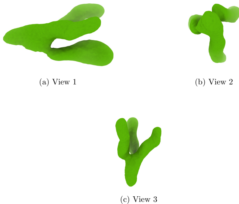
Figure 4: Isosurface at threshold=0.034400. Views generated by ChimeraX at a the following X, Y, Z angles: View 1 (0, -90, -90), View 2 (-90, 0, -90), View 3 (0, 0, 0).
