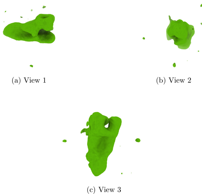
Figure 4: Isosurface at threshold=0.009250. Views generated by ChimeraX at a the following X, Y, Z angles: View 1 (0, -90, -90), View 2 (-90, 0, -90), View 3 (0, 0, 0).
