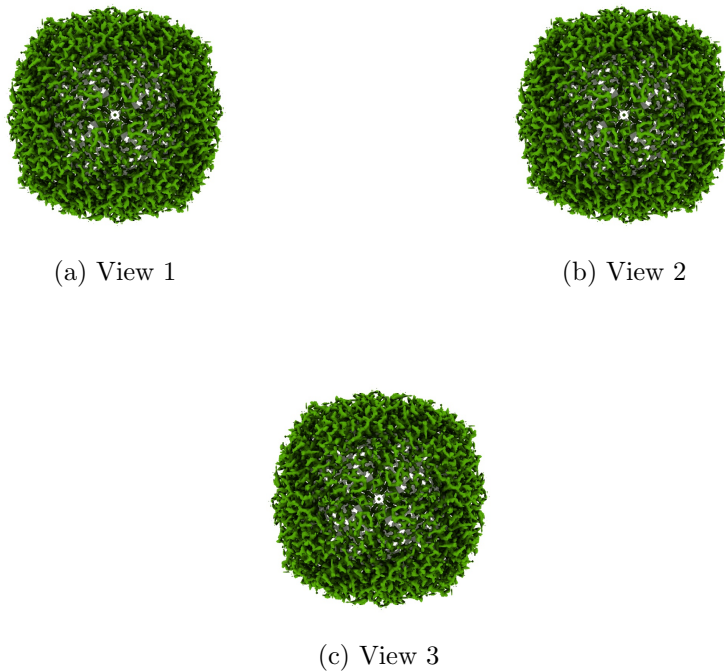
Figure 4: Isosurface at threshold=0.628000. Views generated by ChimeraX at a the following X, Y, Z angles: View 1 (0, -90, -90), View 2 (-90, 0, -90), View 3 (0, 0, 0).
