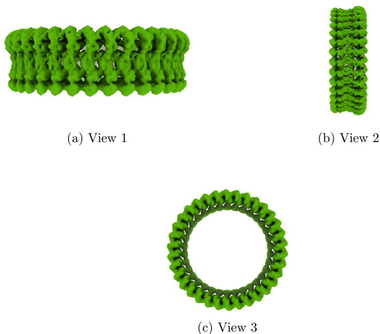
Figure 4: Isosurface at threshold=0.144000. Views generated by ChimeraX at a the following X, Y, Z angles: View 1 (0, -90, -90), View 2 (-90, 0, -90), View 3 (0, 0, 0).
