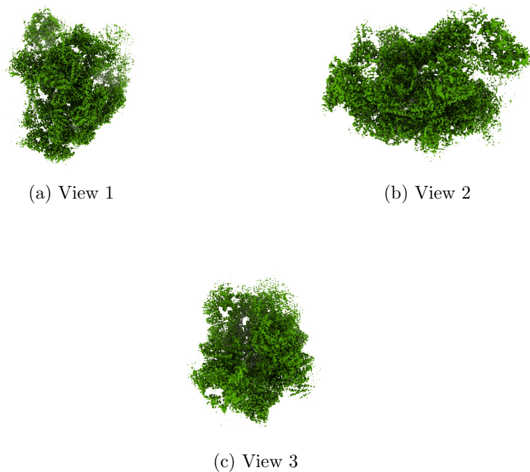
Figure 4: Isosurface at threshold=0.981000. Views generated by ChimeraX at a the following X, Y, Z angles: View 1 (0, -90, -90), View 2 (-90, 0, -90), View 3 (0, 0, 0).
