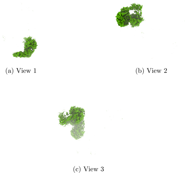
Figure 4: Isosurface at threshold=0.452000. Views generated by ChimeraX at a the following X, Y, Z angles: View 1 (0, -90, -90), View 2 (-90, 0, -90), View 3 (0, 0, 0).
