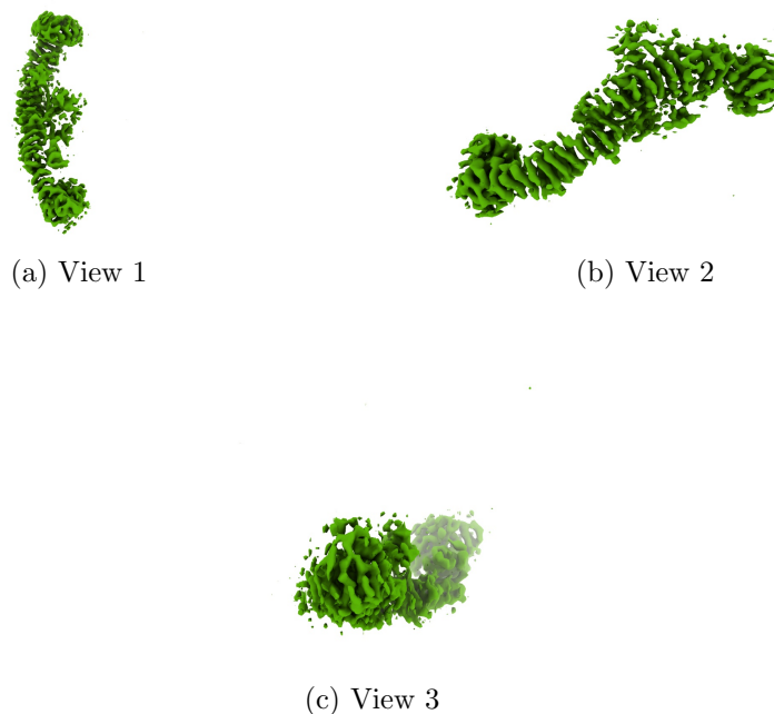
Figure 4: Isosurface at threshold=0.574000. Views generated by ChimeraX at a the following X, Y, Z angles: View 1 (0, -90, -90), View 2 (-90, 0, -90), View 3 (0, 0, 0).
