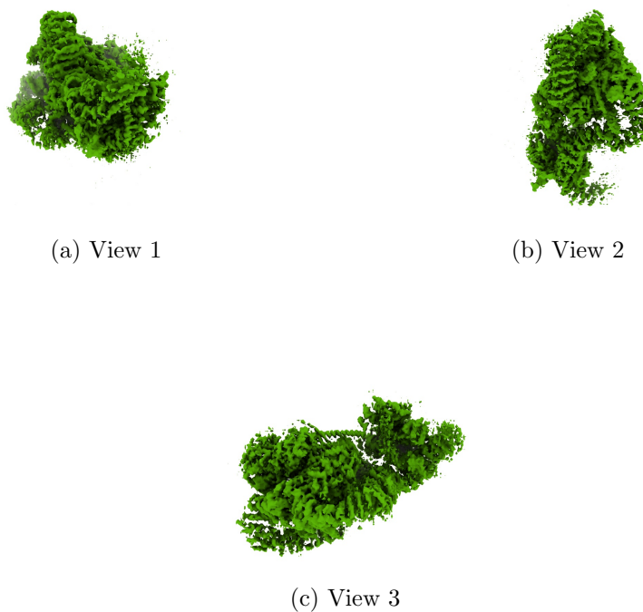
Figure 4: Isosurface at threshold=0.573500. Views generated by ChimeraX at a the following X, Y, Z angles: View 1 (0, -90, -90), View 2 (-90, 0, -90), View 3 (0, 0, 0).
