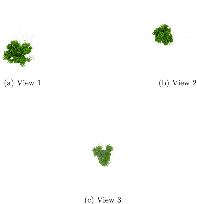
Figure 4: Isosurface at threshold=0.728000. Views generated by ChimeraX at a the following X, Y, Z angles: View 1 (0, -90, -90), View 2 (-90, 0, -90), View 3 (0, 0, 0).
