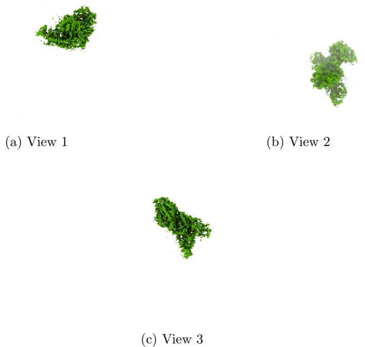
Figure 4: Isosurface at threshold=0.727800. Views generated by ChimeraX at a the following X, Y, Z angles: View 1 (0, -90, -90), View 2 (-90, 0, -90), View 3 (0, 0, 0).
