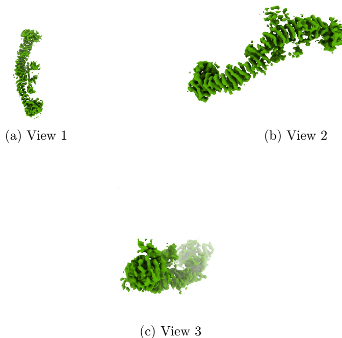
Figure 4: Isosurface at threshold=0.574000. Views generated by ChimeraX at a the following X, Y, Z angles: View 1 (0, -90, -90), View 2 (-90, 0, -90), View 3 (0, 0, 0).
