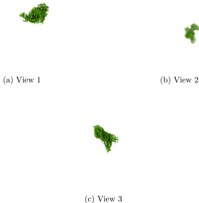
Figure 4: Isosurface at threshold=0.883000. Views generated by ChimeraX at a the following X, Y, Z angles: View 1 (0, -90, -90), View 2 (-90, 0, -90), View 3 (0, 0, 0).
