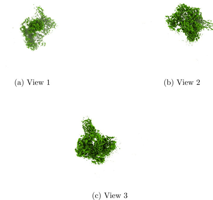
Figure 4: Isosurface at threshold=0.571000. Views generated by ChimeraX at a the following X, Y, Z angles: View 1 (0, -90, -90), View 2 (-90, 0, -90), View 3 (0, 0, 0).
